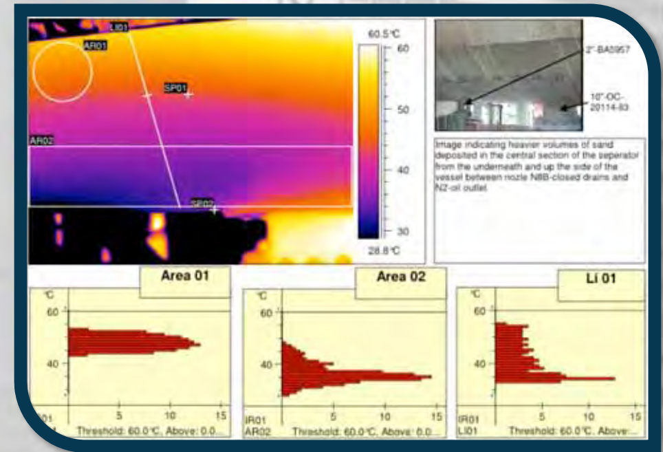
Thermo imaging of a knockout tank at a refinery
